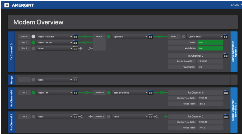
Overview Window
